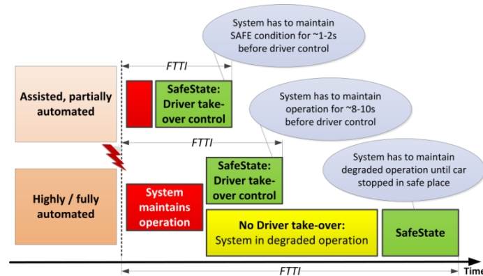
Figure 6: Different concepts for transition to safe state.
